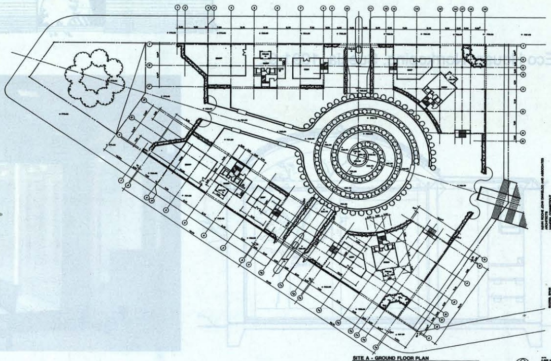
SITE A - GROUND FLOOR PLAN
